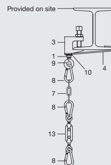
KN 88 Minimum suspension height without link chain: 389 mm Article number: 505340
