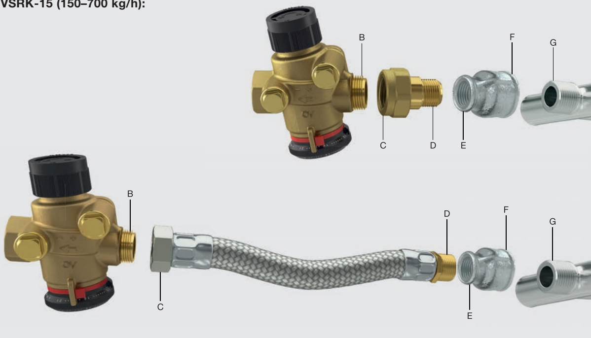
Example of VSRK-15 (150–700 kg/h): Flow
