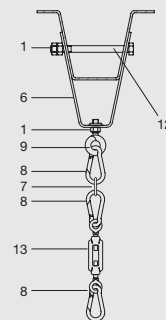
KN 86 Minimum suspension height without link chain: 421 mm Article number: 505280
