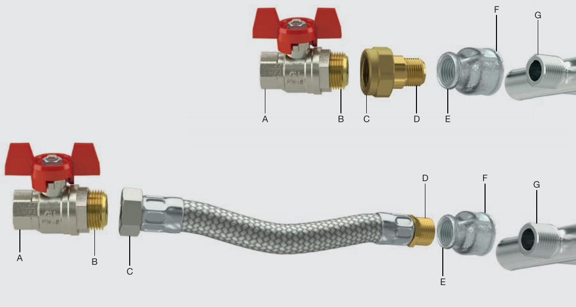
Example of VSRK-15 (150–700 kg/h): Flow
