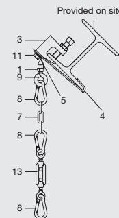
KN 87 Minimum suspension height without link chain: 410 mm Article number: 505290
